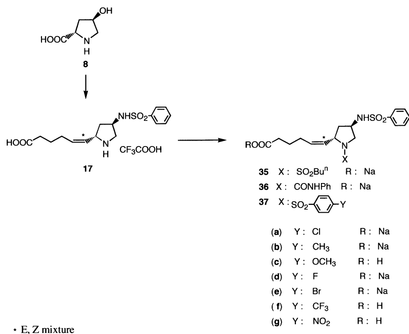
Scheme 3. (a) \text{SOCl}_2 , MeOH; (b) \text{PhSO}_2\text{Cl} , \text{Et}_3\text{N} , \text{CH}_2\text{Cl}_2 ; (c) \text{MsCl} , \text{Et}_3\text{N} , \text{CH}_2\text{Cl}_2 ; (d) \text{BzONa} , DMSO; (e) \text{K}_2\text{CO}_3 , MeOH; (f) \text{NaN}_3 , DMSO; (g) \text{H}_2 -Pd/C, MeOH; (h) DIBAL, toluene, -78^\circ\text{C} ; (i) \text{HOOC}(\text{CH}_2)_4\text{P}^+\text{Ph}_3\text{Br}^- , t\text{-BuOK} , DMAC; (j) 1\text{N-NaOH} , MeOH.
