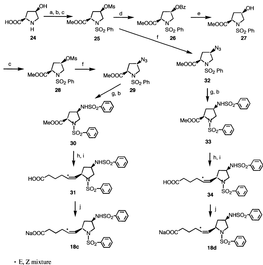
Scheme 3. (a) \text{SOCl}_2 , MeOH; (b) \text{PhSO}_2\text{Cl} , \text{Et}_3\text{N} , \text{CH}_2\text{Cl}_2 ; (c) \text{MsCl} , \text{Et}_3\text{N} , \text{CH}_2\text{Cl}_2 ; (d) \text{BzONa} , DMSO; (e) \text{K}_2\text{CO}_3 , MeOH; (f) \text{NaN}_3 , DMSO; (g) \text{H}_2 -Pd/C, MeOH; (h) DIBAL, toluene, -78^\circ\text{C} ; (i) \text{HOOC}(\text{CH}_2)_4\text{P}^+\text{Ph}_3\text{Br}^- , t\text{-BuOK} , DMAC; (j) 1\text{N-NaOH} , MeOH.
